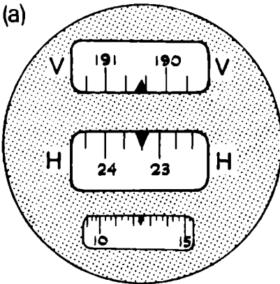
Example of horizontal circle reading (Sexagesimal)
