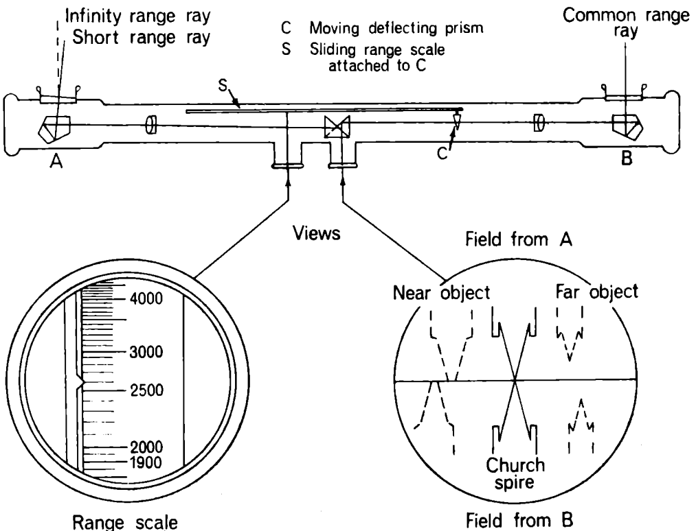
Fig. 5. The range finder
