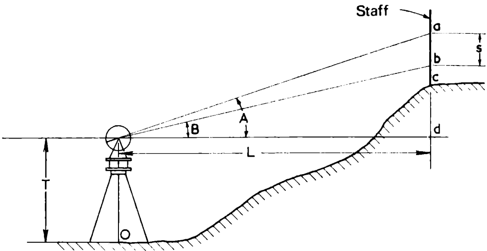
Fig. 7. Tangential tacheometry
