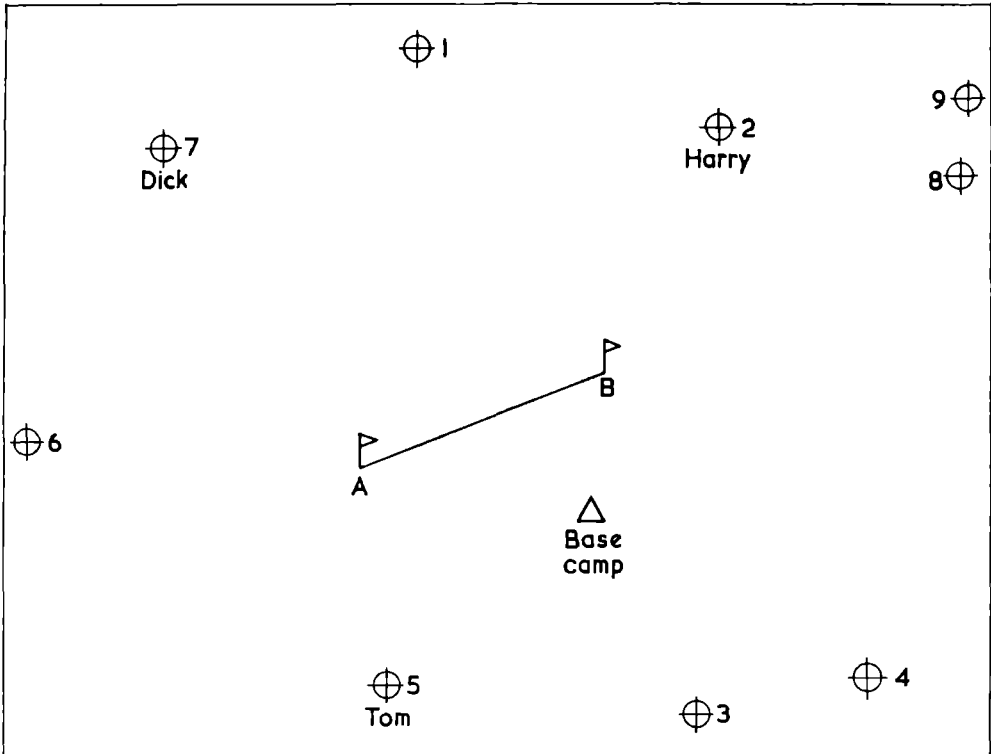
Fig. 1. A possible major control scheme
