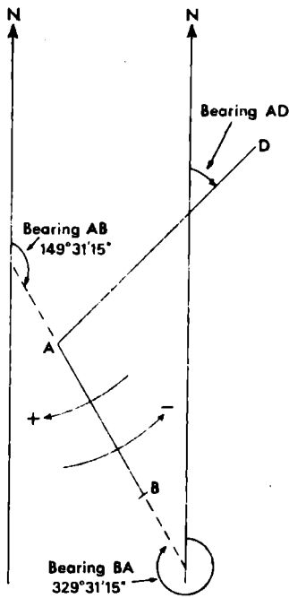
Fig. 15. Grid bearings (a) typical grid network (b) notation for bearings
