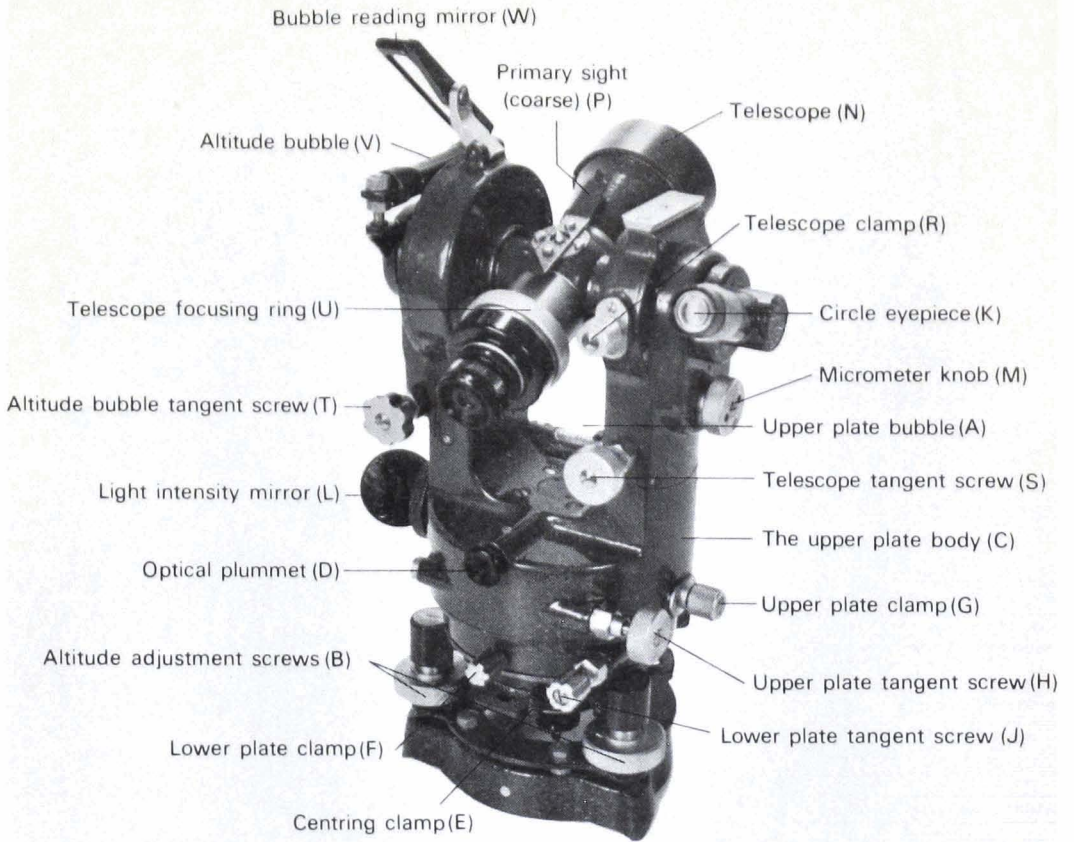
Important features of the microptic theodolite
