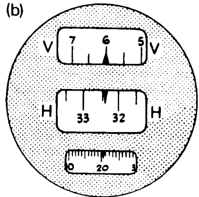
Example of vertical reading (Centesimal)
